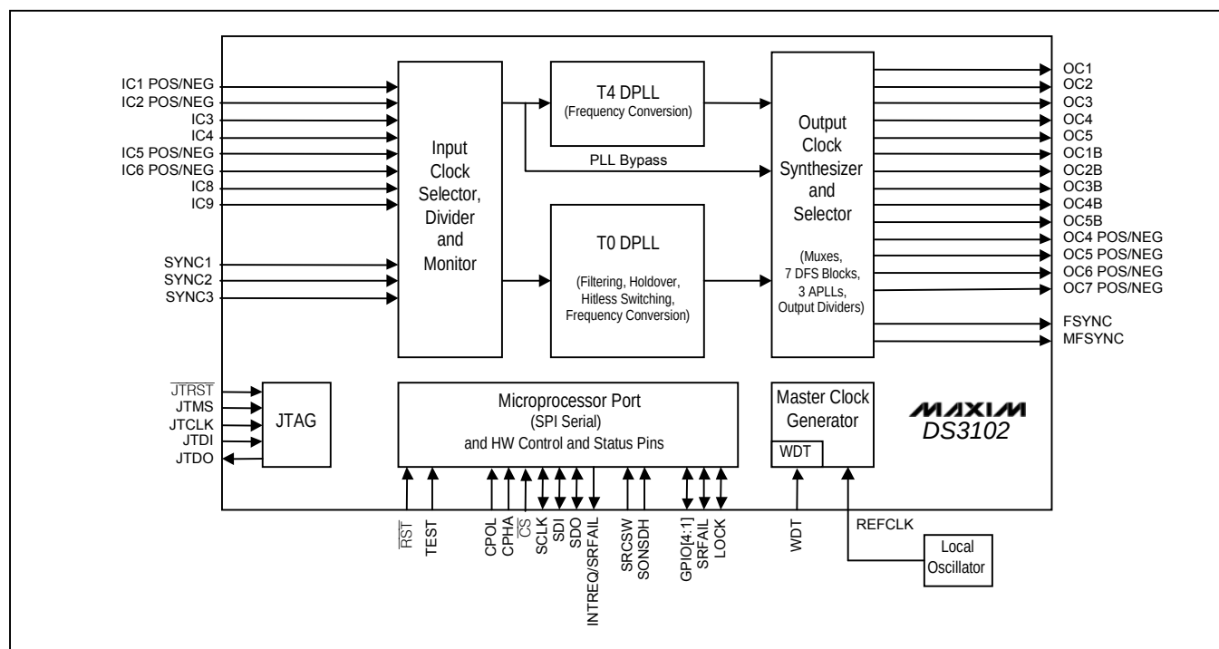
Figure 3-1. Block Diagram
